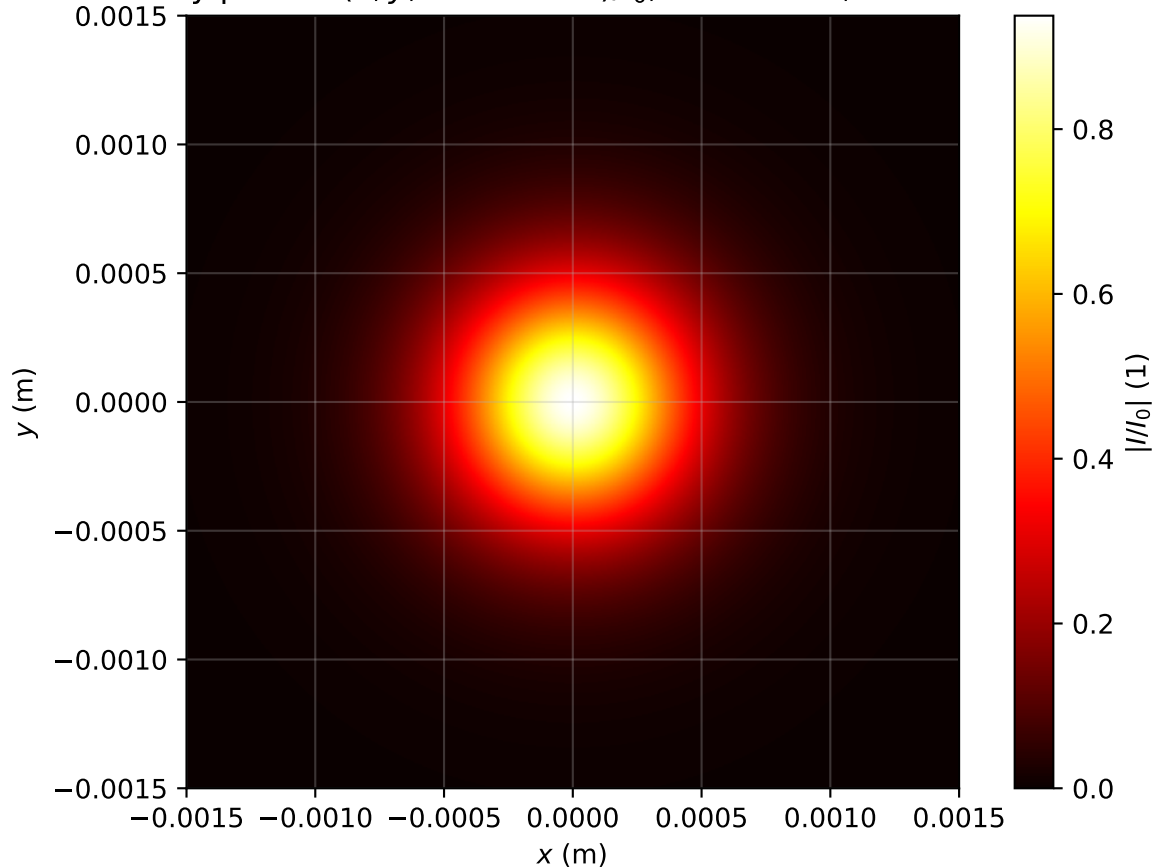
Intensity profile I(x, y, z = 2.627m)/I_0 , Pin=0.7Pcr, artificial time
